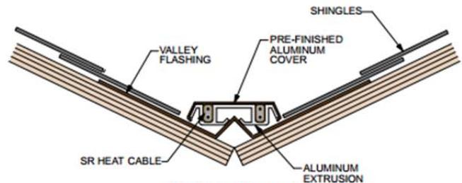
Valley Panel
