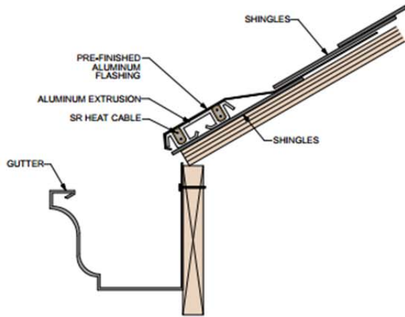
Eave Panel
